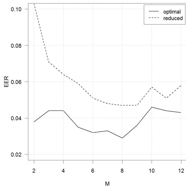
Figure 2: Equal error rates for different numbers of mixture components M
