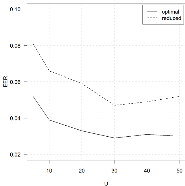
Figure 1: Equal error rates for different numbers of UBM speakers U
